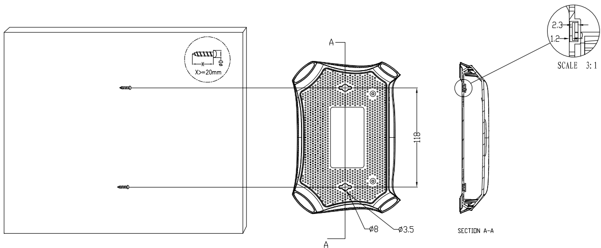
Figure 2-2 Wall-mount Install
