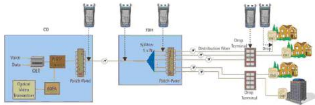
Figure 4-3 Measurement points of the optical power in the GPON network
