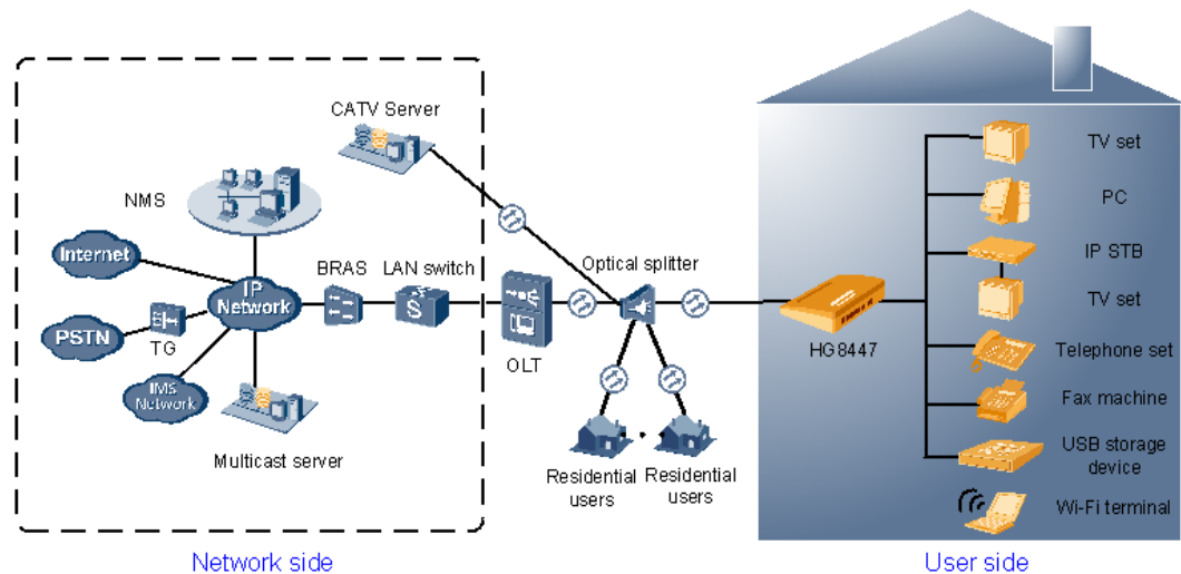
Figure 2-30 Network topology of the HG8447
