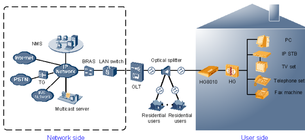
Figure 2-25 Network topology of the HG8010
