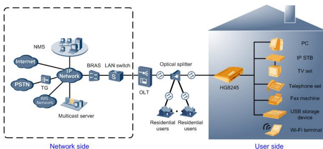
Figure 2-28 Network topology of the HG8245
