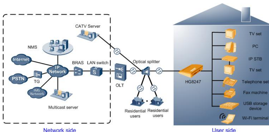
Figure 2-29 Network topology of the HG8247
