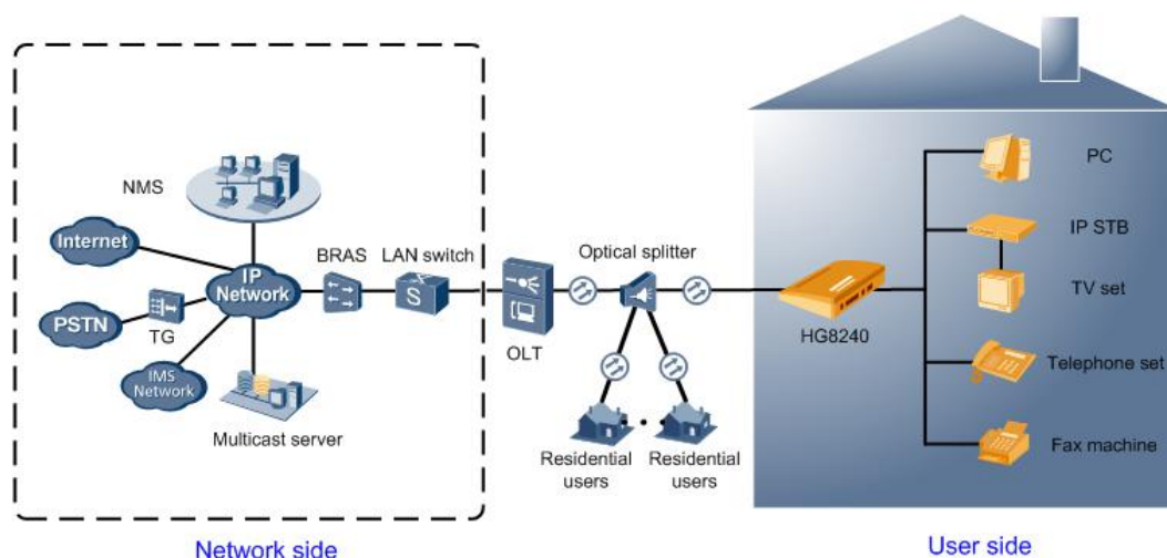
Figure 2-27 Network topology of the HG8240
