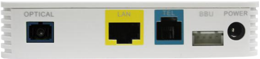
Figure 2-9 Ports on the rear panel of the HG8110
