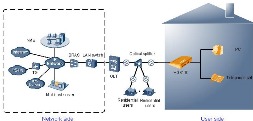
Figure 2-26 Network topology of the HG8110
